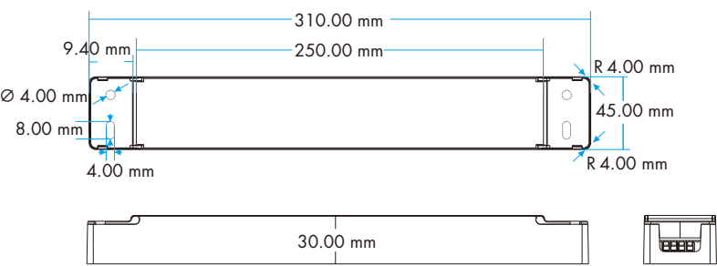
(Product size)
