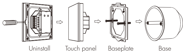
Installation diagram:
