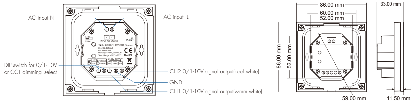
Installation diagram:
