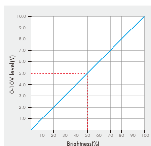
0-10V Dimmer
