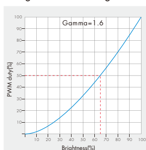
Logarithmic dimming curve
