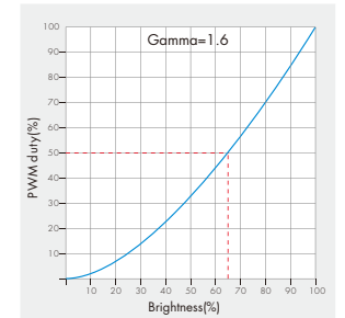
Dimming curve for RGB/RGB/DIM
