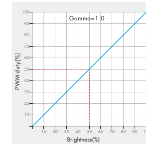
Dimming curve for CCT
